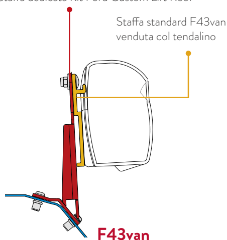
Staffa dedicata Kit Ford Custom Lift Roof
