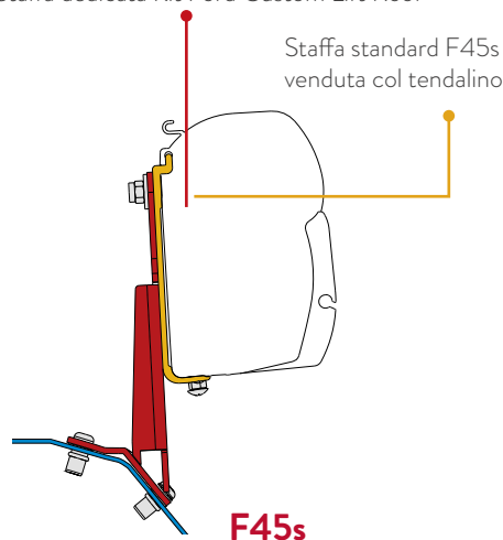
Staffa dedicata Kit Ford Custom Lift Roof
