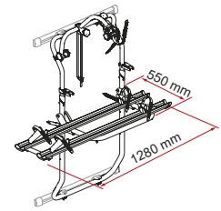
Carry-Bike DJ
