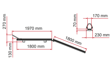
Carry-Moto
