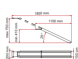
Carry-Ramp
