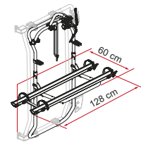
Carry-Bike Frame
